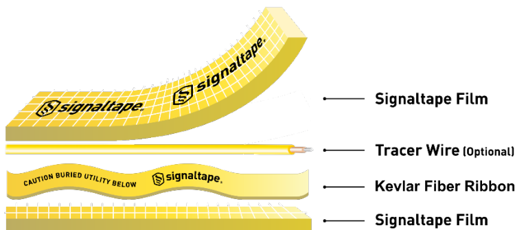
Signaltape® Exploded Drawing
